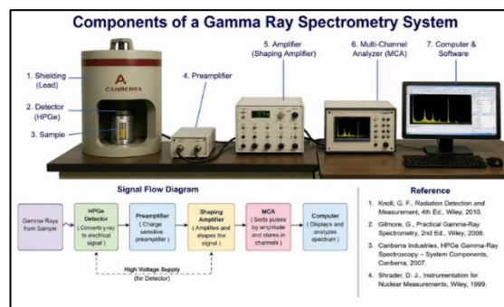
Figure 2: Showing component of Gamma-ray spectrometry (Knoll,2010)
